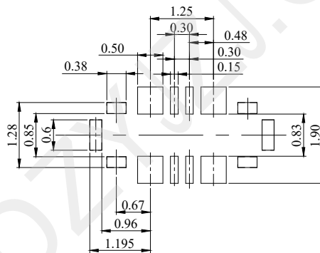
RECOMMENDED METAL DIMENSIONS (THICKNESS: 0.10 mm) DIMENSIONAL TOLERANCE: ±0.01
