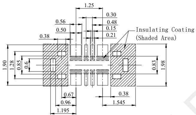
RECOMMENDED PCB LAYOUT DIMENSIONAL TOLERANCE: ±0.02
