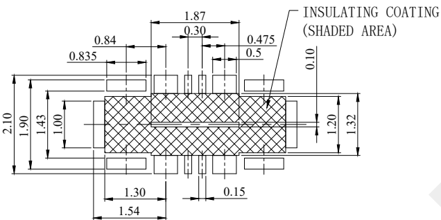
RECOMMENDED PCB LAYOUT DIMENSIONAL TOLERANCE: ±0.03
