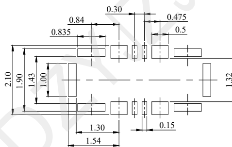
RECOMMENDED METAL DIMENSIONS (THICKNESS: 0.08 mm) DIMENSIONAL TOLERANCE: ±0.01
